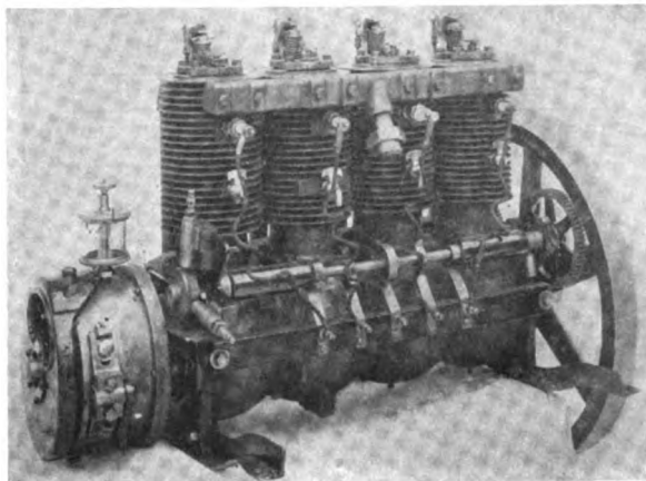
First Franklin Motor, without Auxillary Valves.
